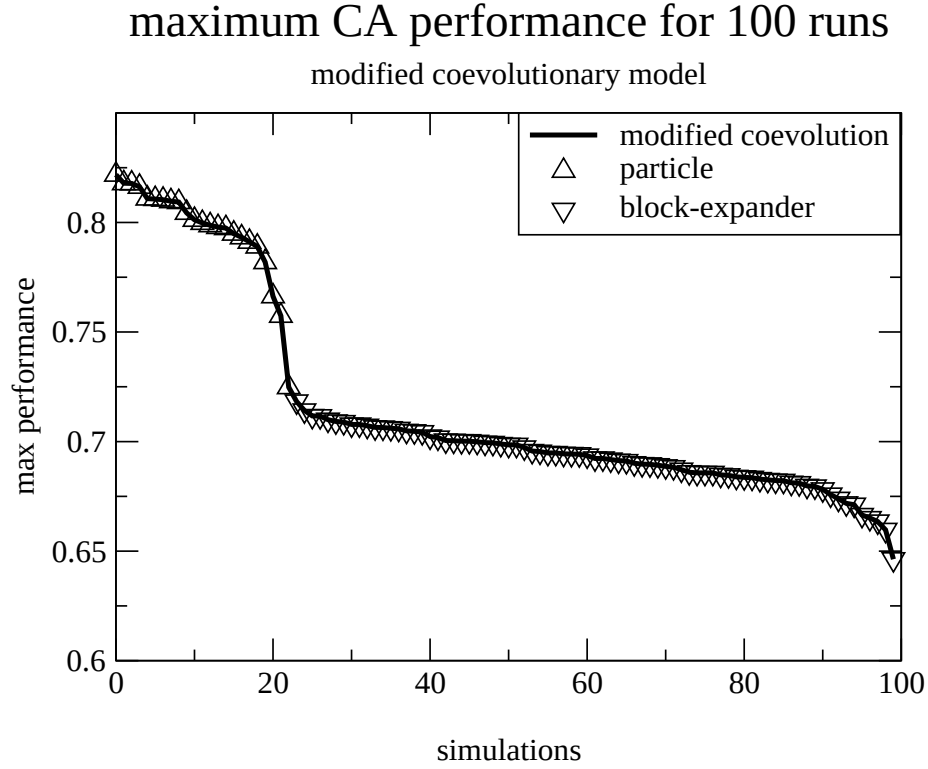
Figure 6: The maximum CA performance found for each of the 100 runs in the modified coevolutionary model. Although the efficacy of the modified model drops sharply, the performance of particle CAs that evolve in this model tend to be somewhat higher than that of the particle CAs that evolve in the original coevolutionary model.
